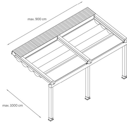
Three Modules 900 cm > 1300 cm Three Modules with one motor & 4 rafters
